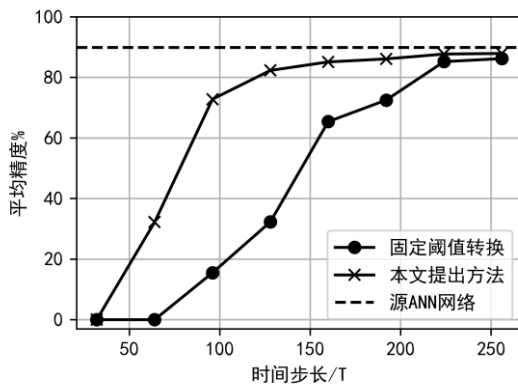
Fig 7 Detection performance of transformed brain-inspired spiking network in RSOD dataset
