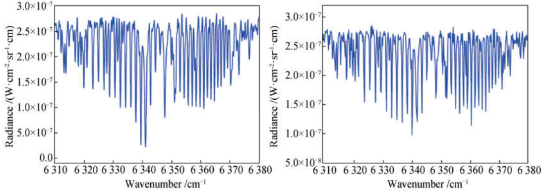
图 5 GMI-I 实测光谱（左）与 GOSAT 光谱（右）比对 Fig. 5 Comparison CO 2 band spectrum of GMI (left) and GOSAT (right)
