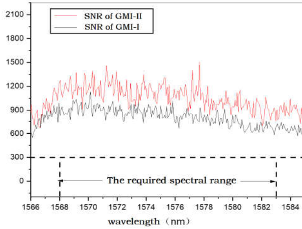
图 6 GMI-II 与 GMI-I 实测光谱域信噪比曲线 Fig. 6 The measured spectral SNR curves of GMI-II and GMI-I
