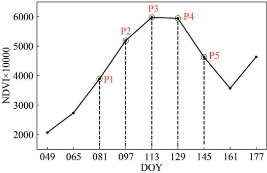
图4 冬小麦关键生长时段划分示意图 Fig. 4 Division of key growth periods of winter wheat
