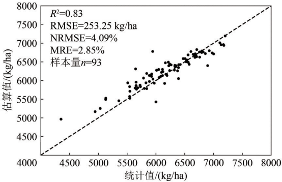
图8 最优模型在验证数据集的观测值和估计产量之间的线性回归 Fig. 8 Linear regression between observed and estimated yield for the validation data set from the optimal model
