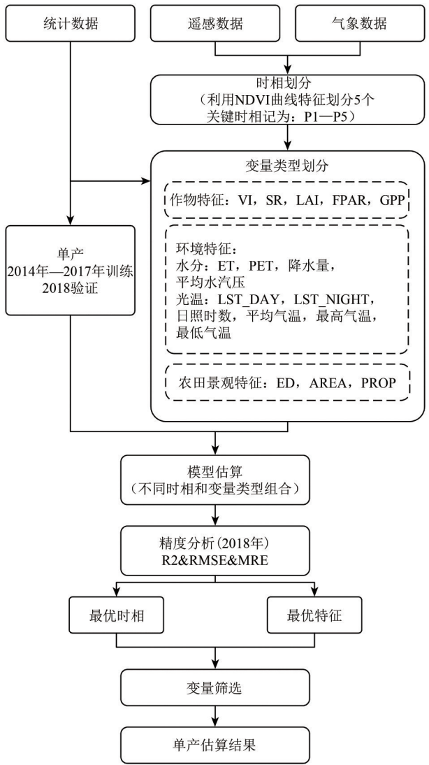
图3 县级产量估算的方法概述 Fig. 3 Overview of methods for estimating county-level wheat yield
