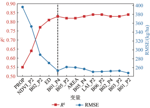
图7 随机森林变量累加分析结果图 Fig. 7 Cumulative analysis results of random forest variables
